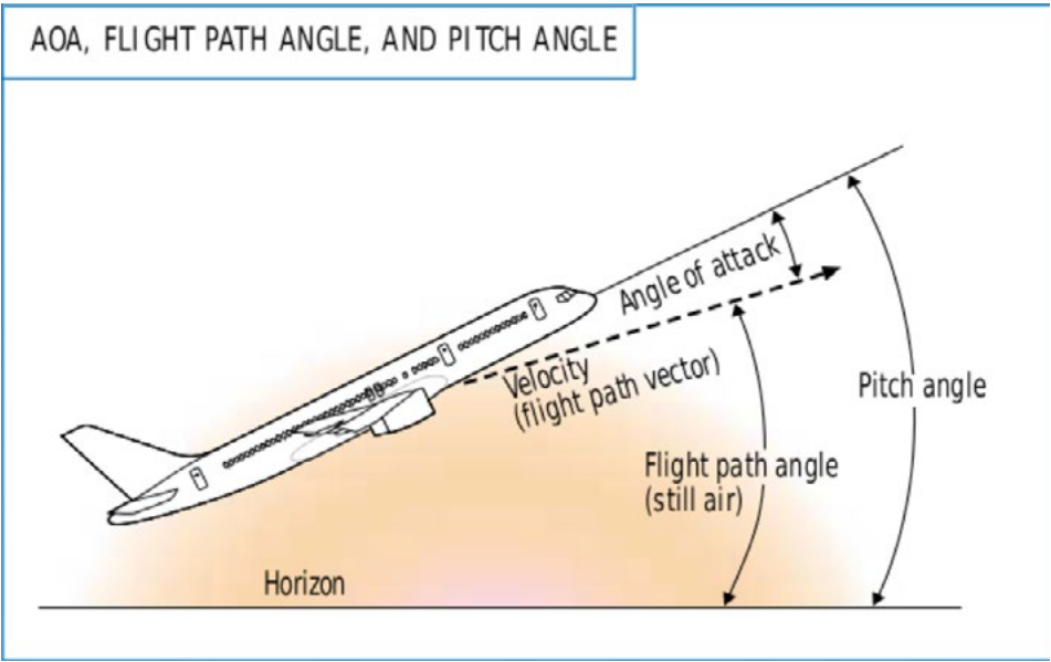
Figure 3 Stall (Reference: https://www.skybrary.aero/index.php/Stall )
